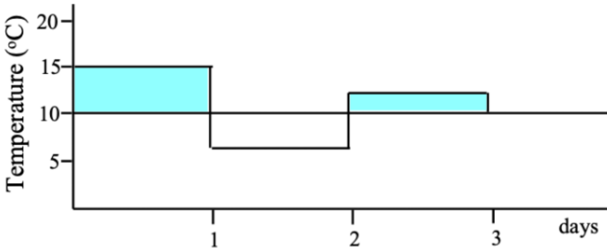
Figure 4: Accumulation at day-degrees at different temperatures
