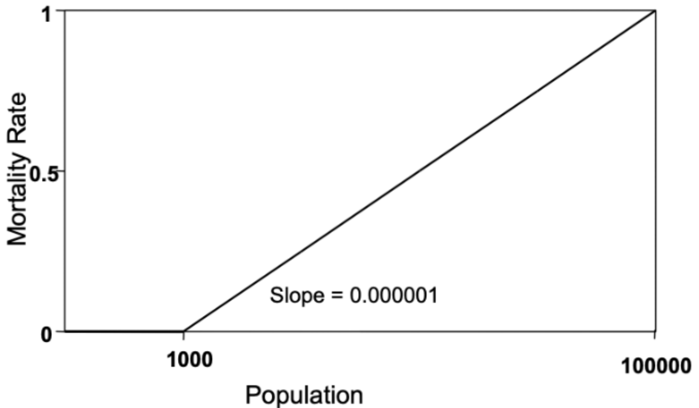
Figure 7: Density-dependent mortality function
