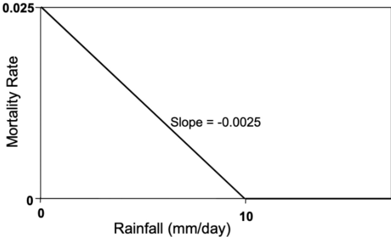
Figure 8: Mortality rate as a function of Rainfall
