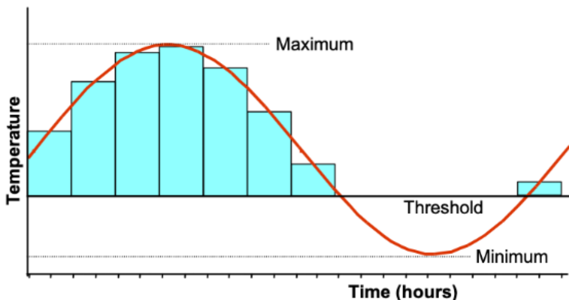
Figure 6: Circadian cycle between daily maximum and minimum temperatures, and the 3-hourly degree-day summation
