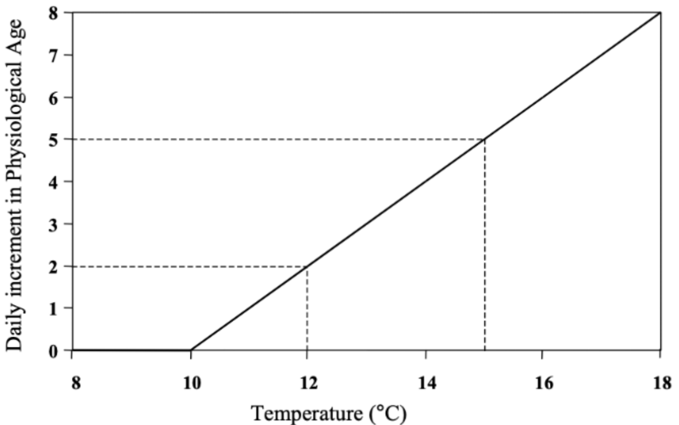
Figure 5: Daily increment in Physiological Age with “Linear above Threshold” function
