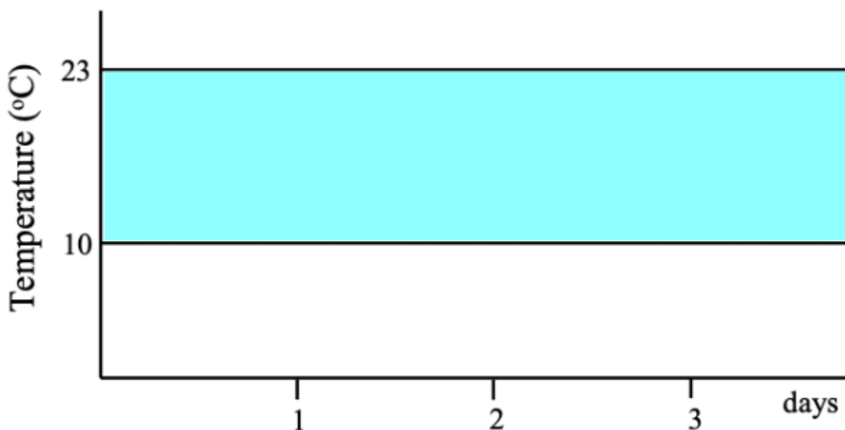
Figure 3: Accumulation of "Day-degrees" at a constant temperature
