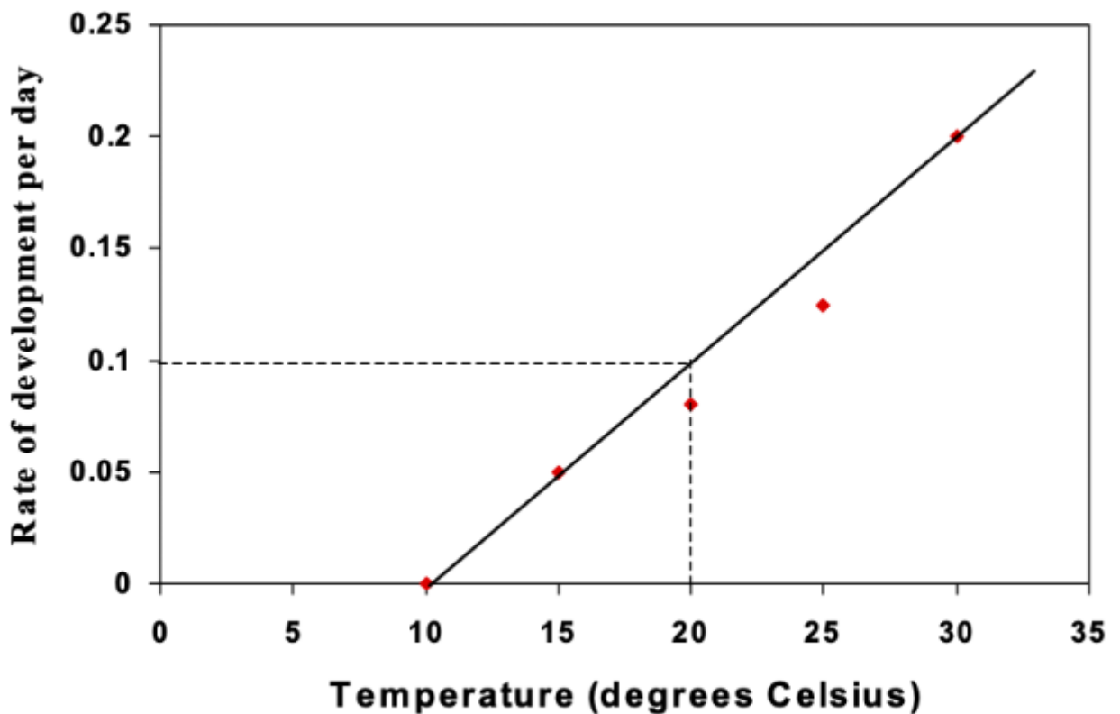
Figure 2-1 Rate of development of juvenile Pseudo-aphids
